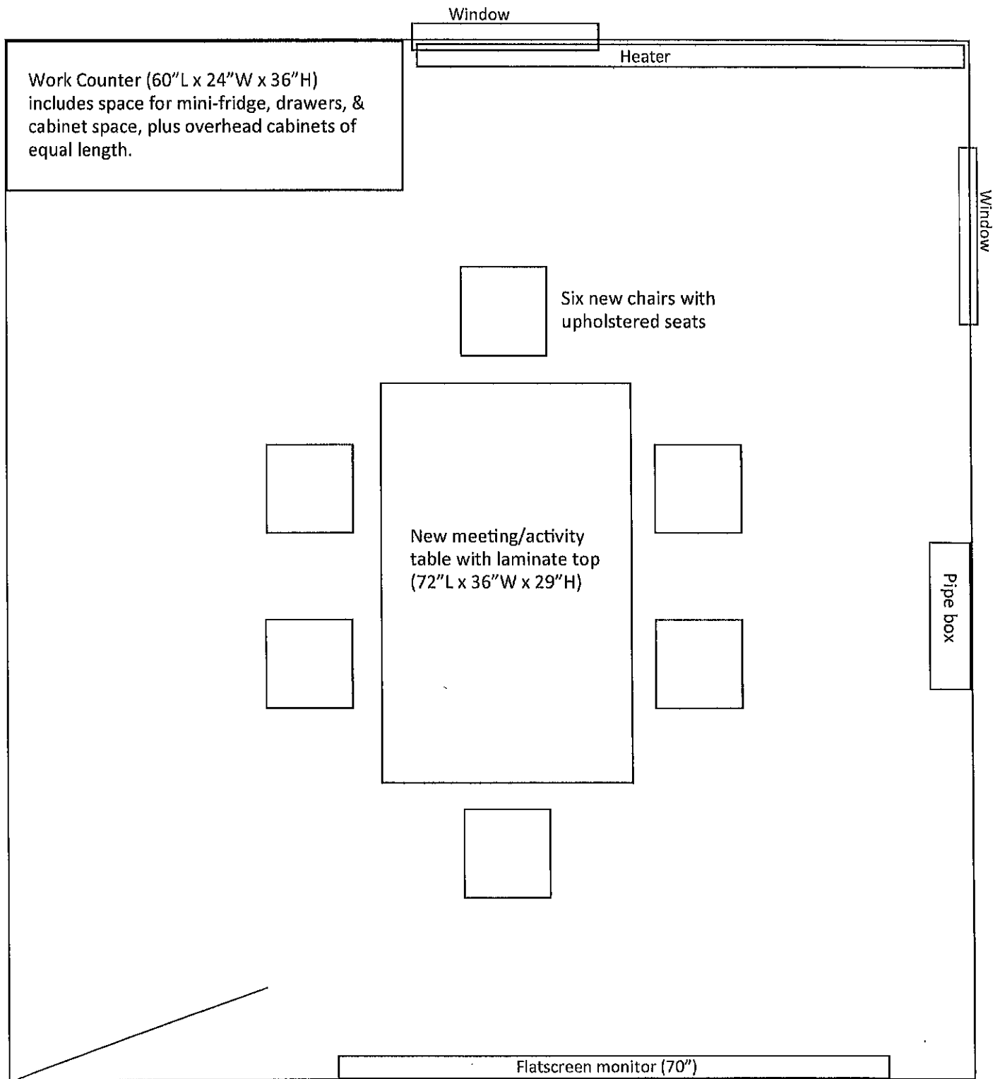
Community Room Floor Plan (Room dimensions 14 x 16 feet - not to scale).
